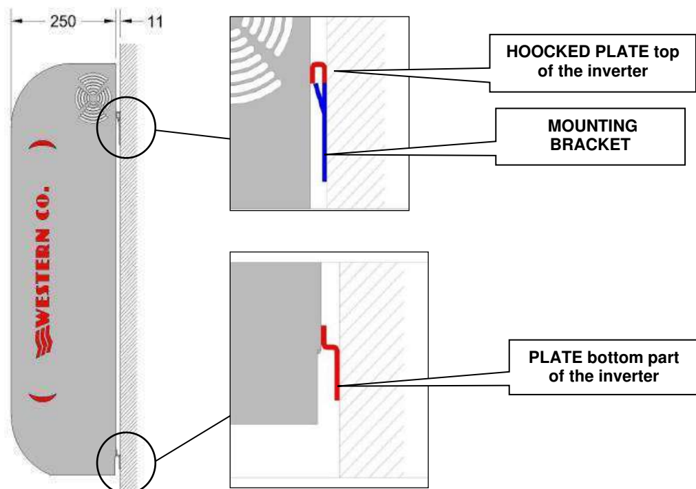
Pic.10 Wall Mounting
