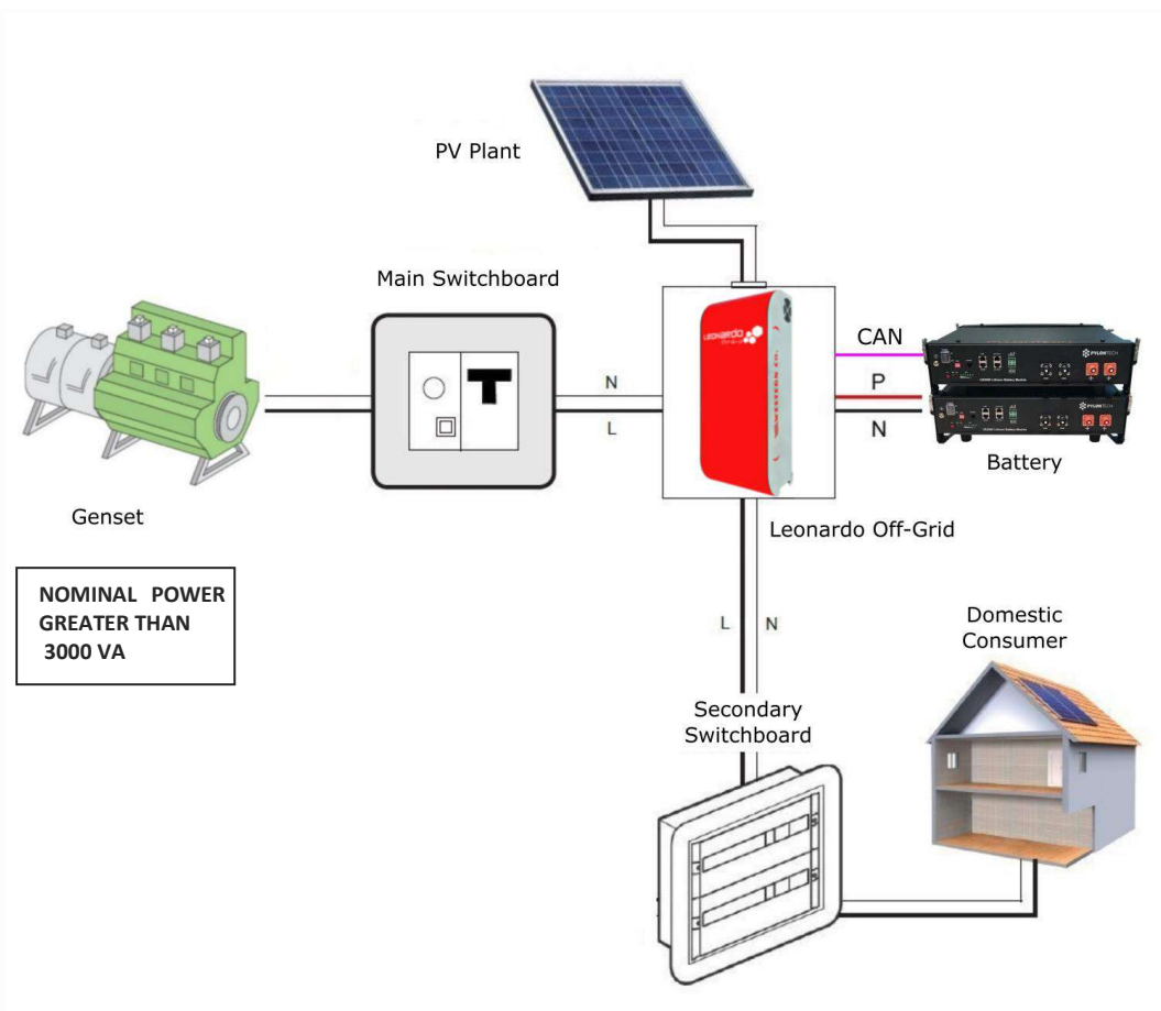
Pic.2 Principle diagram
