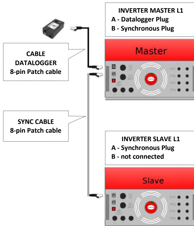
Pic.15 Connection diagram Sync control BUS of the parallel 6 kW system
