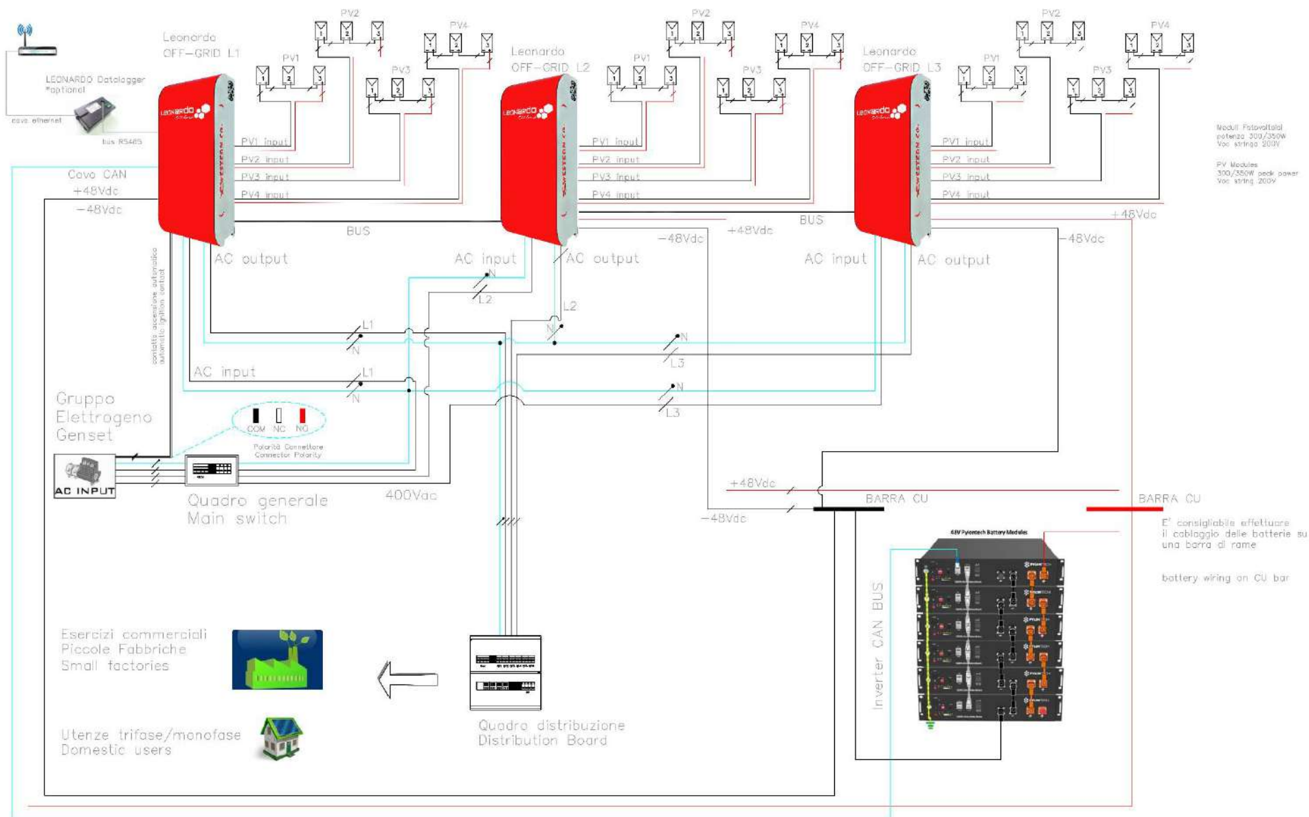
Pic.13 Single line diagram of 9KW three-phase system
