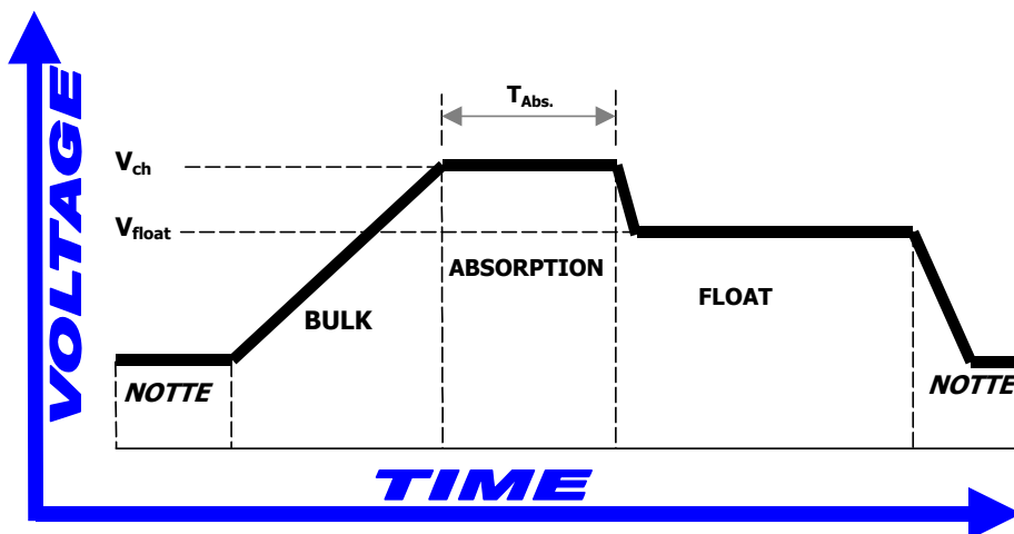
Pic.7 Charging curve
