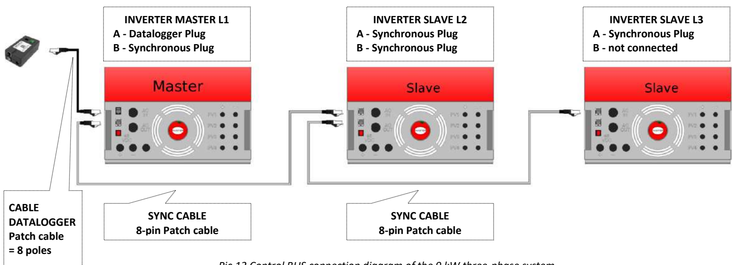
Pic.12 Control BUS connection diagram of the 9 kW three-phase system
