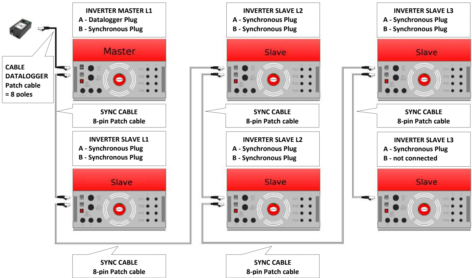
Pic.14 Connection diagram Sync control BUS of the three-phase 18 kW system
