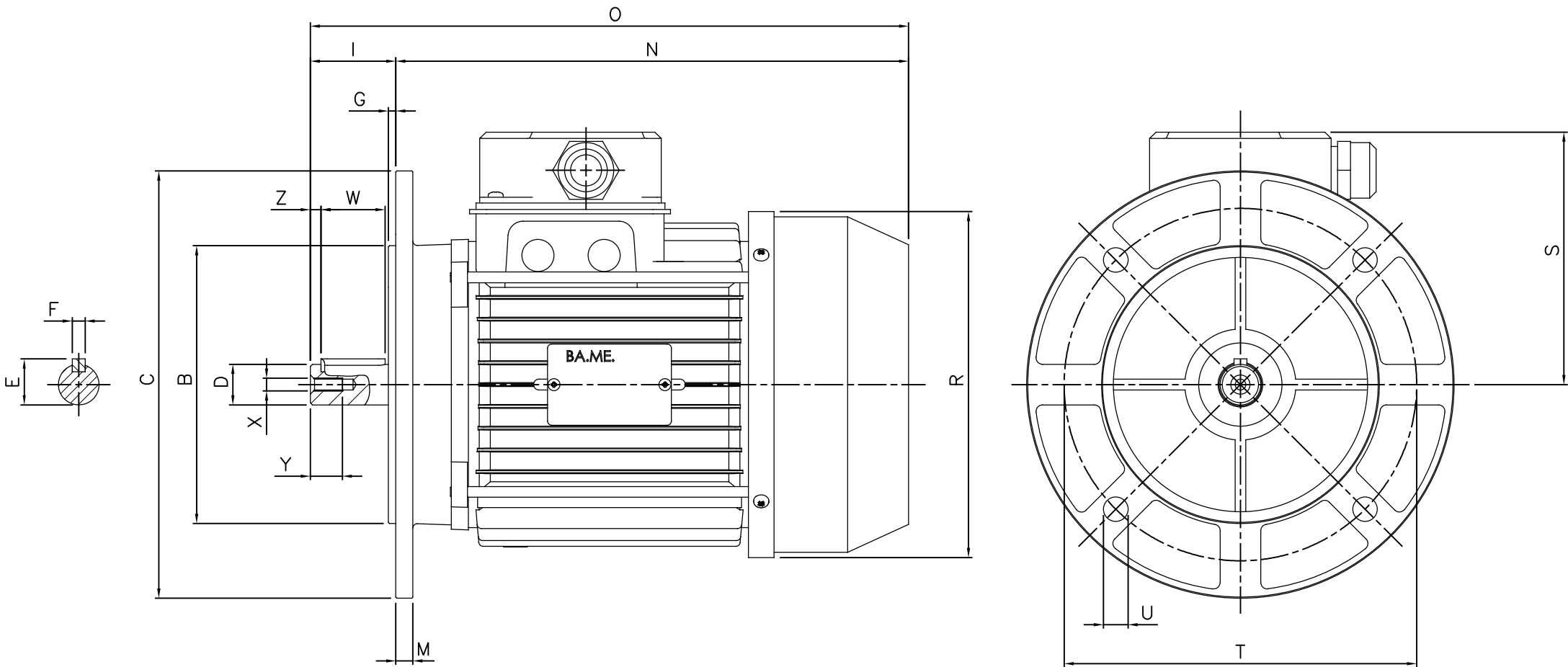
FORMA B5 – DIMENSIONI / FRAME SIZE B5 FORM
