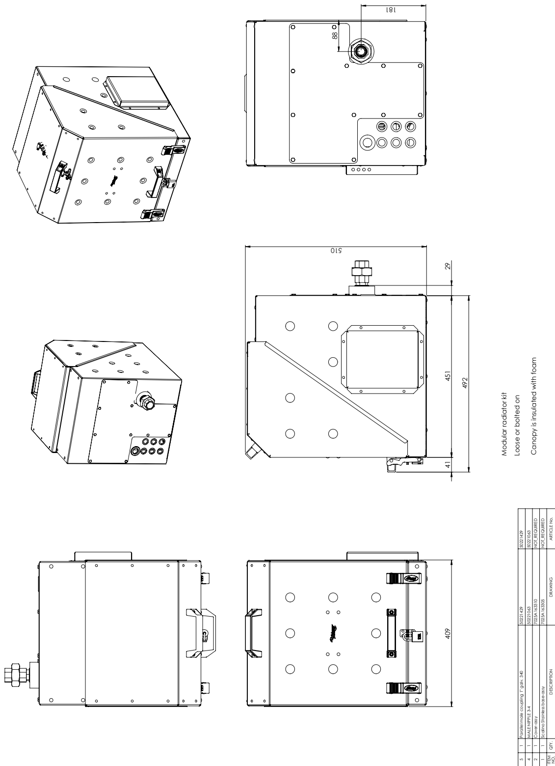
Figure 12: Dimensions
