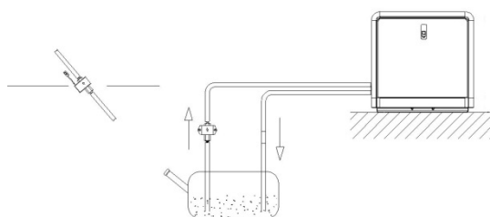
Figure 5: Fuel line assemblies with pump mounted vertically or in an angle
