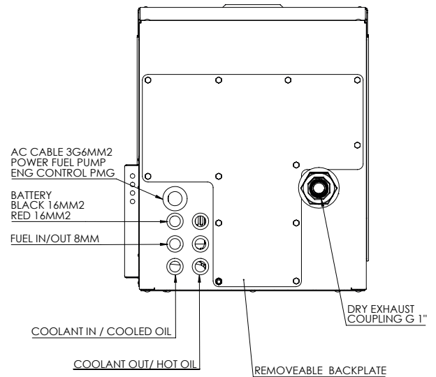
Figure 2: Genverter connections
