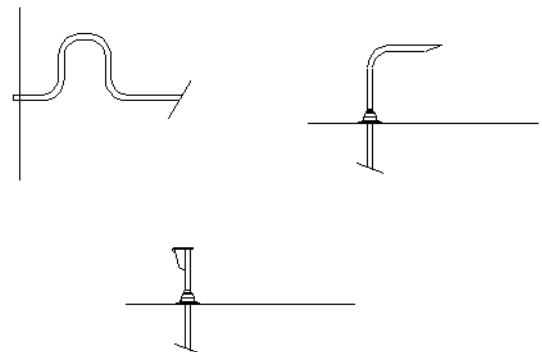
Figure 9: Ways to prevent water from getting in
