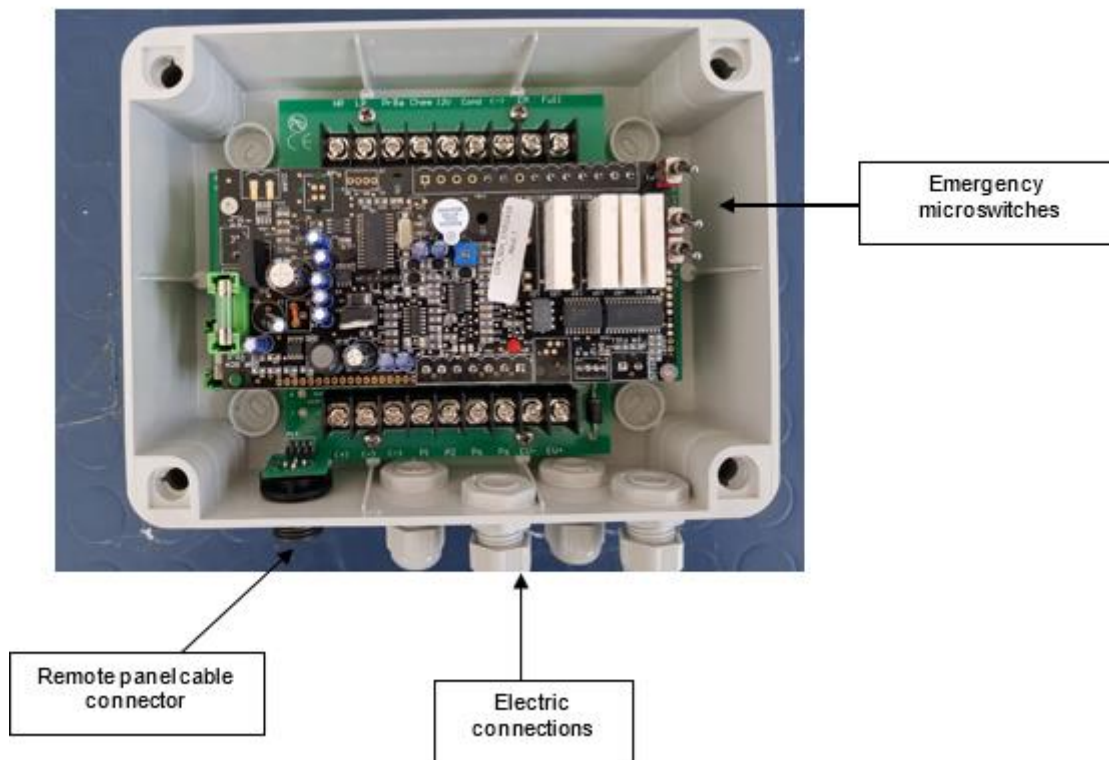
COMPUTER BOX WITH SWITCHES FIG. 3-10
