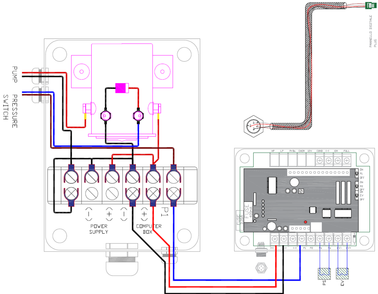
ELECTRIC SCHEME MODULAR 100 12/24V DC FIG. 4-5
